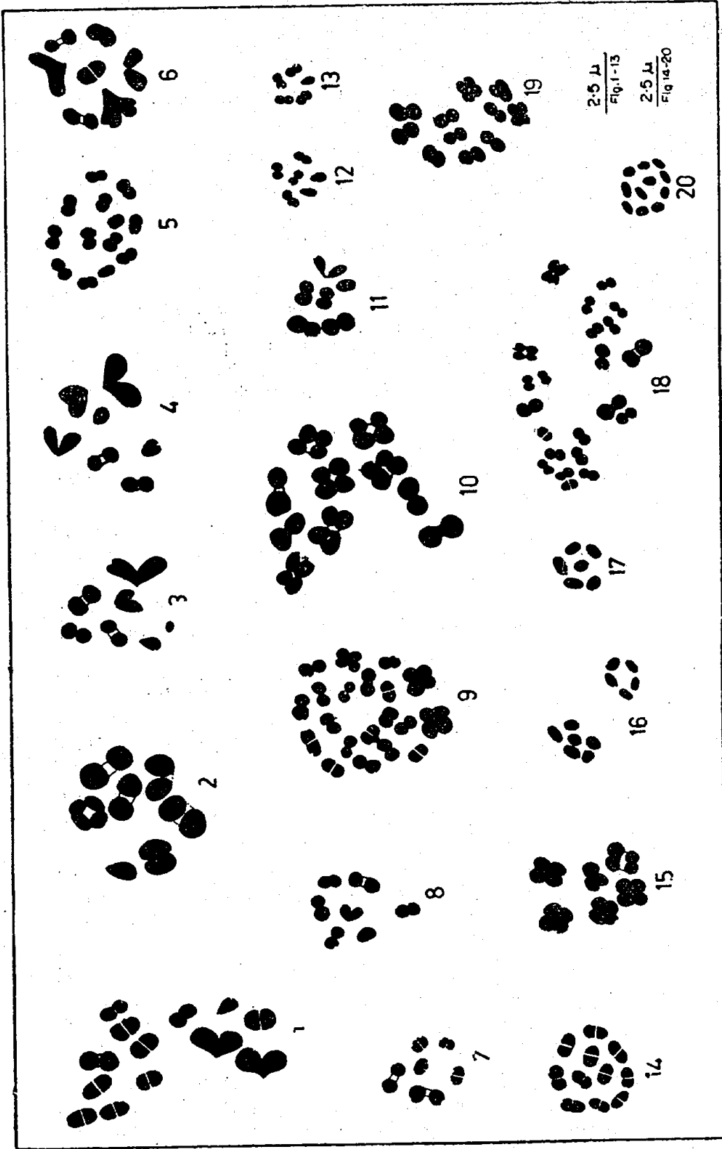
Species: Temora stylifera —Fig. 1 Spermatoonial metaphase, Fig. 2. Metaphase I, Figs. 3 & 4. Metaphases II with 7 chromosomes Species: Temora discaudata —Fig. 5. Spermatoonial metaphase, Fig. 6. Metaphase I, Figs. 7 & 8. Metaphases II with 6 and 7 chromosomes respectively. Species: Lobidocera detruncata —Fig. 9. Spermatoonial metaphase, Fig. 10. Metaphase I. Species: Acartia southwelli —Fig. 11. Spermatoonial metaphase, Fig. 12. Metaphase I, Fig. 13. Metaphase II. Species: Pseudodiaptomus auribilli —Fig. 14. Spermatoonial metaphase, Fig. 15. Metaphase I, Fig. 16. Telophase I showing 5 and 6 chromosomes at the two poles respectively. Species: Pseudodiaptomus serricaudatus —Fig. 18. Spermatoonial metaphase, Fig. 19. Metaphase I, Fig. 20. Metaphase II.
